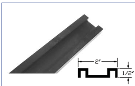
4204100831 Floor Guide Track SPC-18 Bronze
