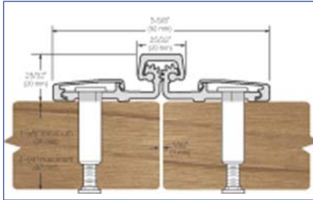
780-057 Series Full Surface Continuous Hinge Reference Drawing
