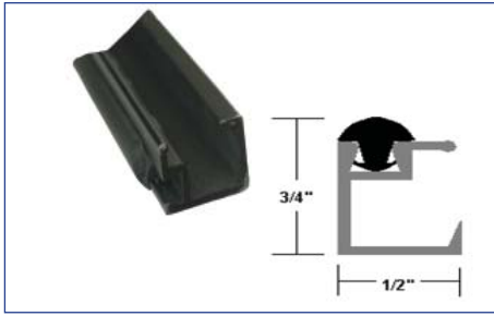
US0101419LLDB 1/4" Glass Stop Bronze
