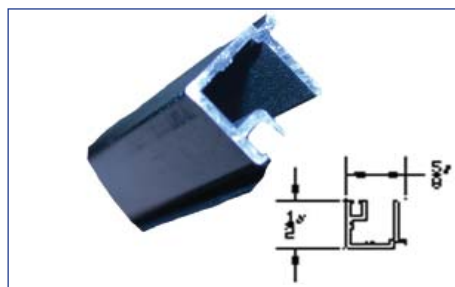
737807 Glass Stop 1/4" Bronze
