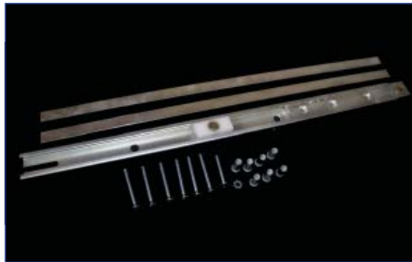
210925 Top Track W/ Pivot & Side Spacers
