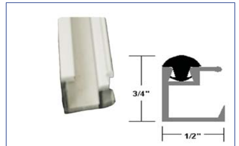
US0101419LLCL 1/4" Glass Stop Clear
