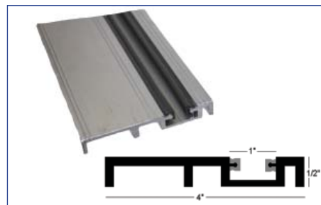
C2873A Threshold/Guide W/ C289 4"
