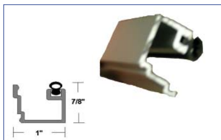
DE021001A 1/4" Clear Glass Stop W/ Vinyl
