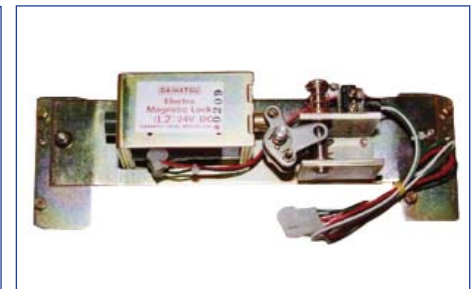
9-99-5563 Fail Safe Lock 1100 L2
