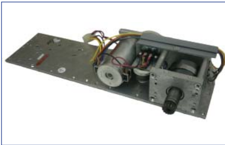
RC7600RO48 Bi-Fold Oper. Assy. RH/OUT 48 Tooth
