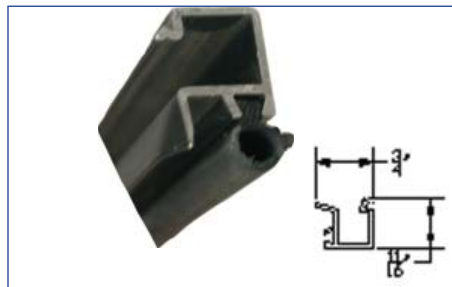
C0338B Glass Stop 1/4" W/ Vinyl Bronze
