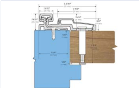
780-210 Full Surface Continuous Reference Drawing
