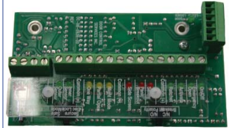
DC08-0936-00 I/O Board
