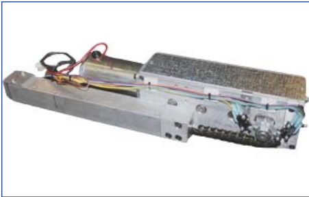
R3500LODDO SW Oper. LH OUT OHC DBL D Shaft
