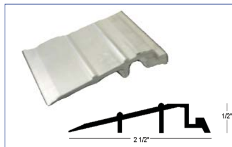
50-01-620 Publix Threshold Lead-Up CL
