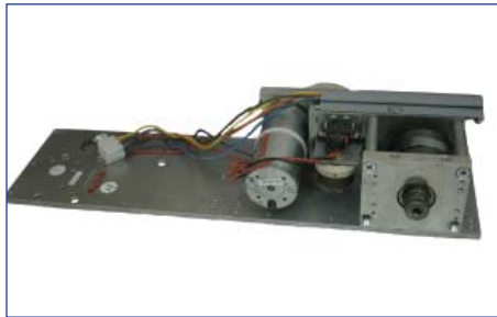
RC7100RO48 Handicap Oper. Assy. RH/OUT 48 Tooth
