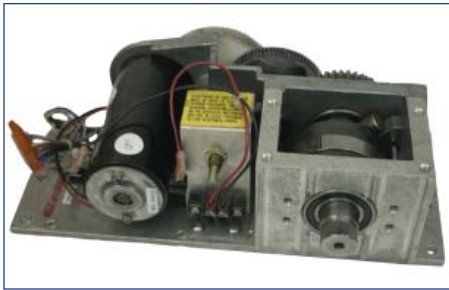
R110378RO Operator RH/OUT
