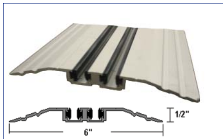
515260 Tapered Threshold 6" Clear
